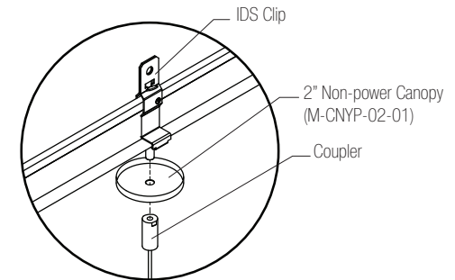
Grid Ceiling
