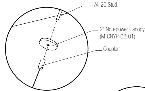
Inaccessible Ceiling
